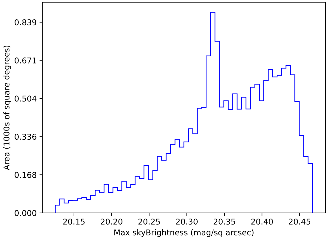
weather_cloudso35v3.4_10yrs WFD i band: Max skyBrightness
