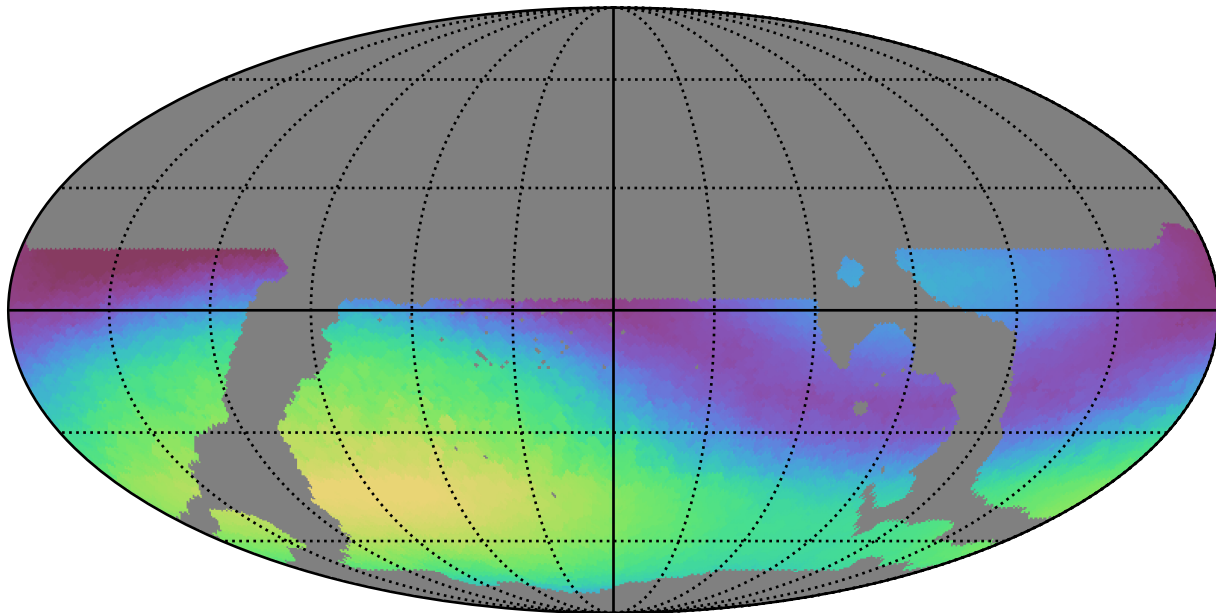
weather_cloudso35v3.4_10yrs WFD g band: Max skyBrightness
