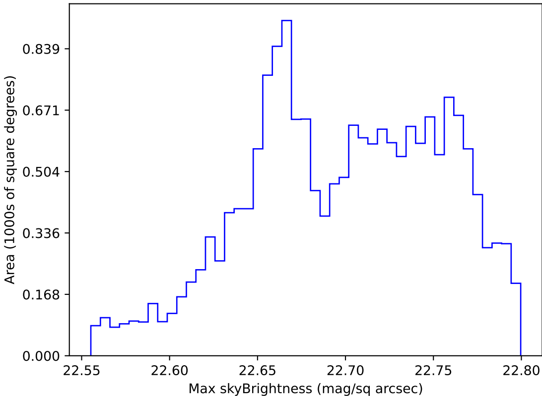
weather_cloudso35v3.4_10yrs WFD all bands: Max skyBrightness
