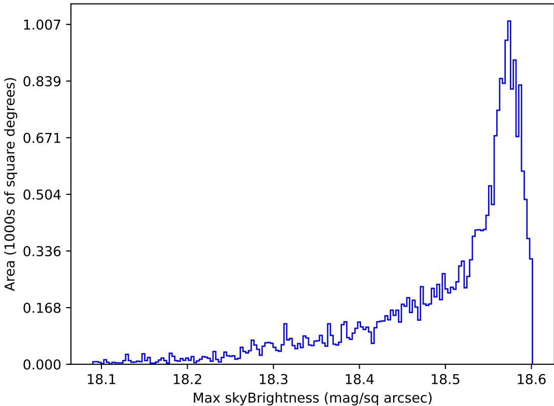
weather_cloudso35v3.4_10yrs All sky y band: Max skyBrightness
