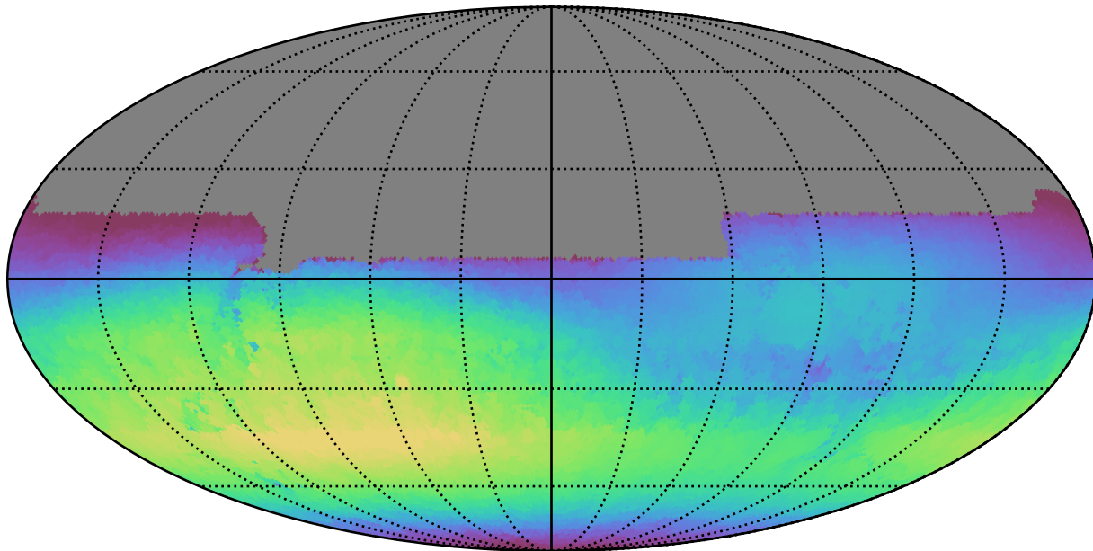
weather_cloudso35v3.4_10yrs All sky u band: Max skyBrightness
