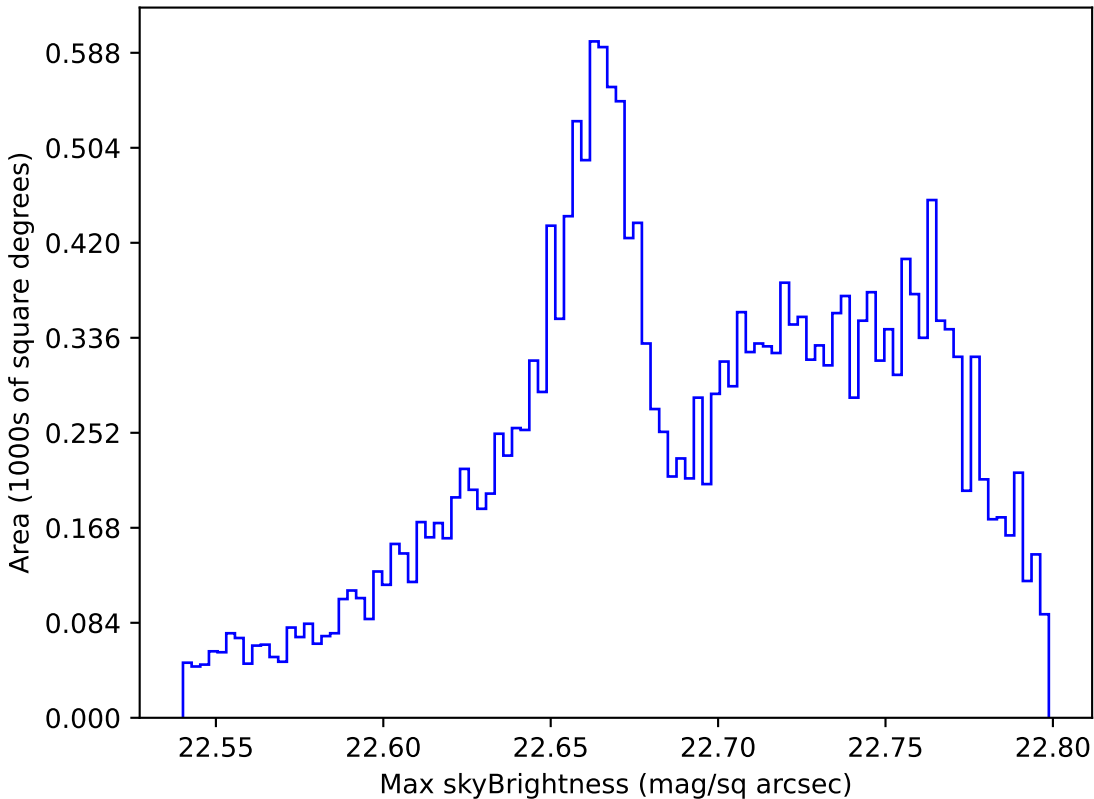
weather_cloudso35v3.4_10yrs All sky u band: Max skyBrightness
