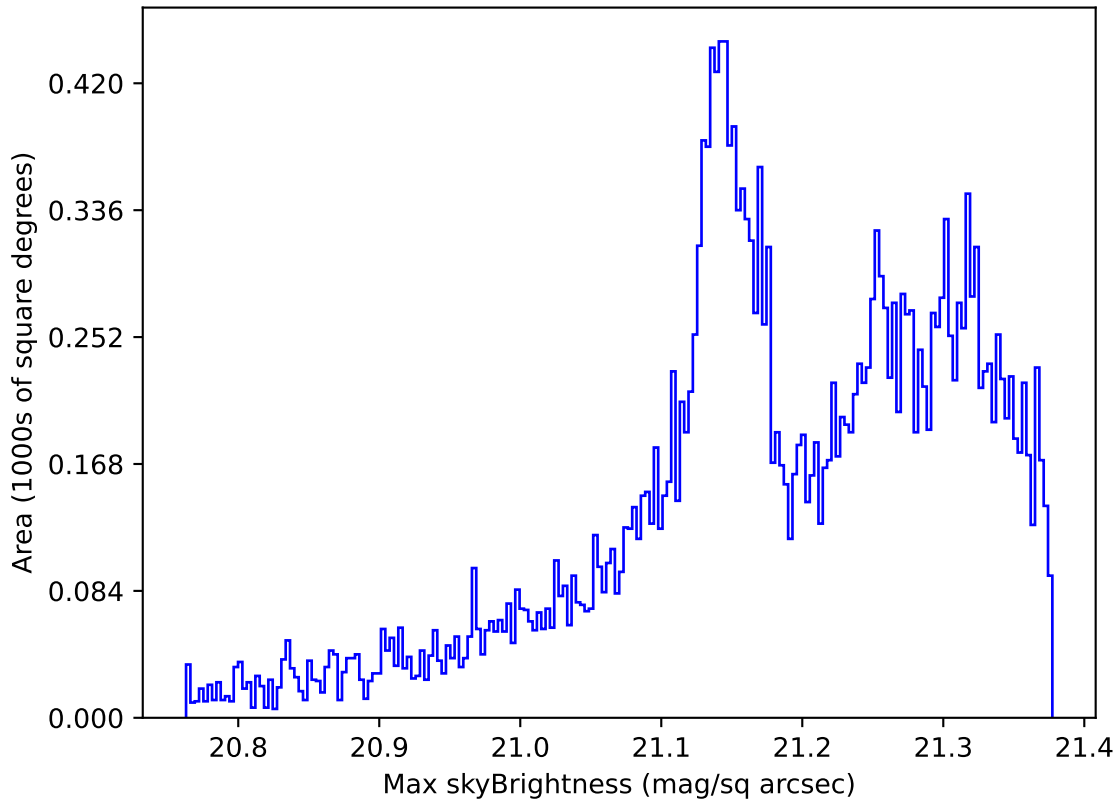
weather_cloudso35v3.4_10yrs All sky r band: Max skyBrightness
