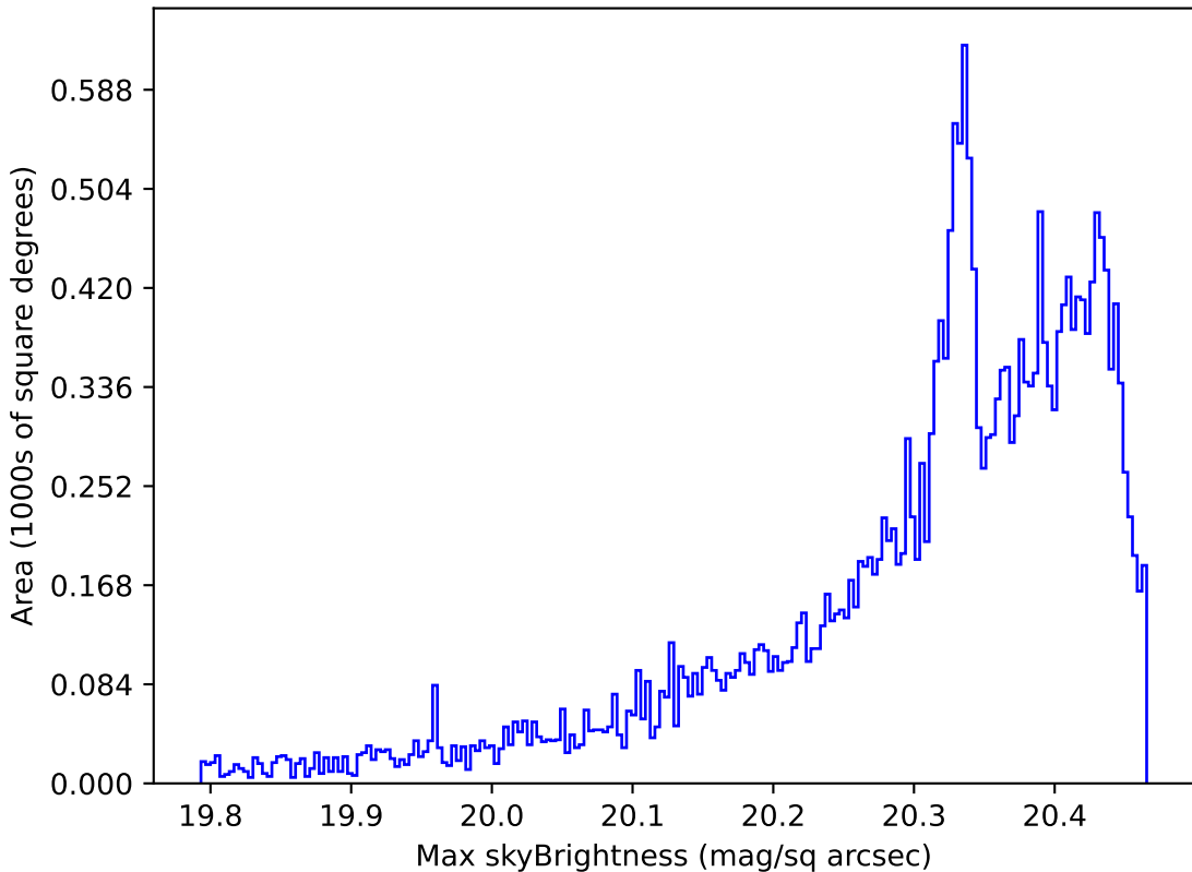
weather_cloudso35v3.4_10yrs All sky i band: Max skyBrightness
