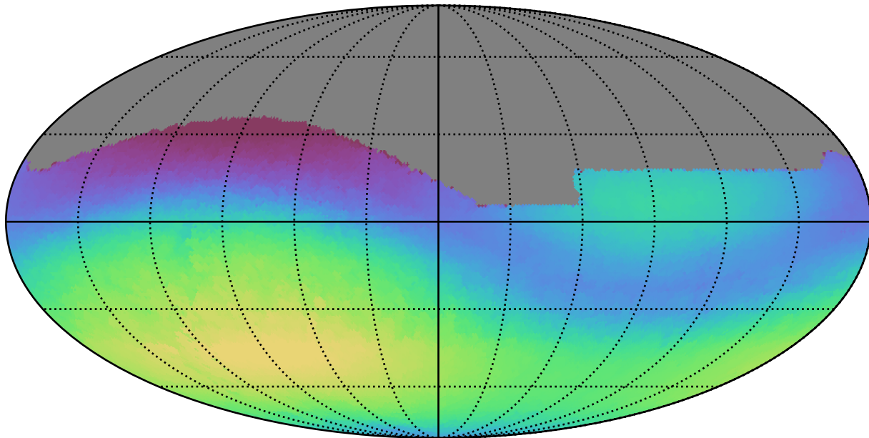
weather_cloudso35v3.4_10yrs All sky g band: Max skyBrightness
