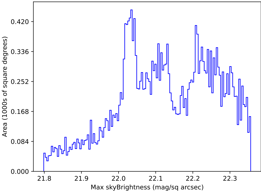
weather_cloudso35v3.4_10yrs All sky g band: Max skyBrightness
