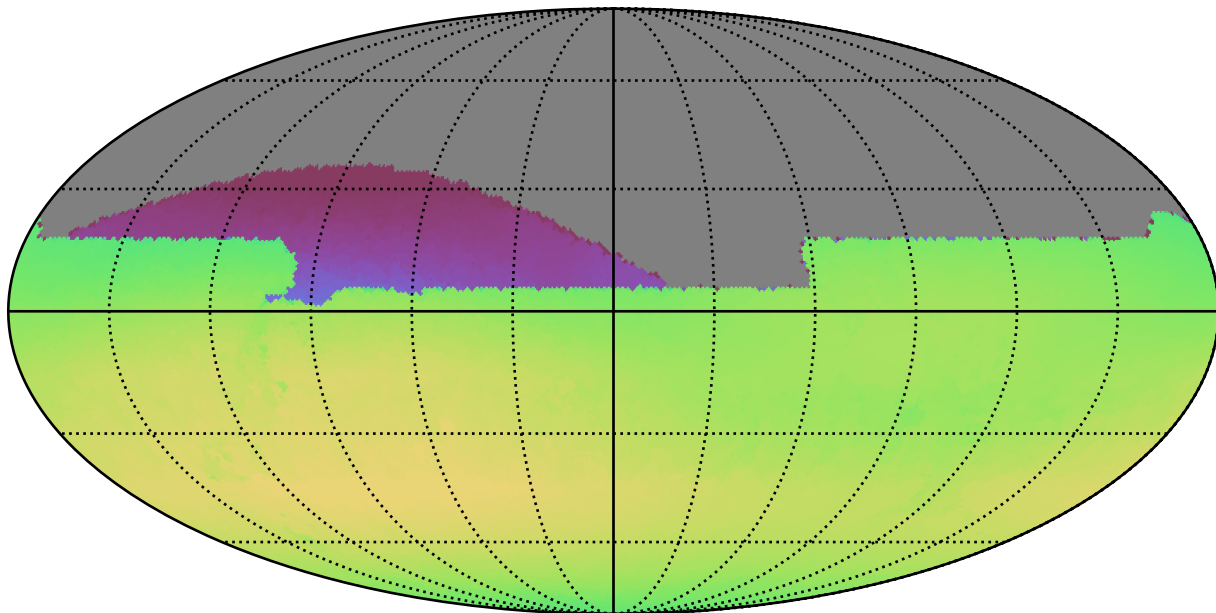
weather_cloudso35v3.4_10yrs All sky all bands: Max skyBrightness
