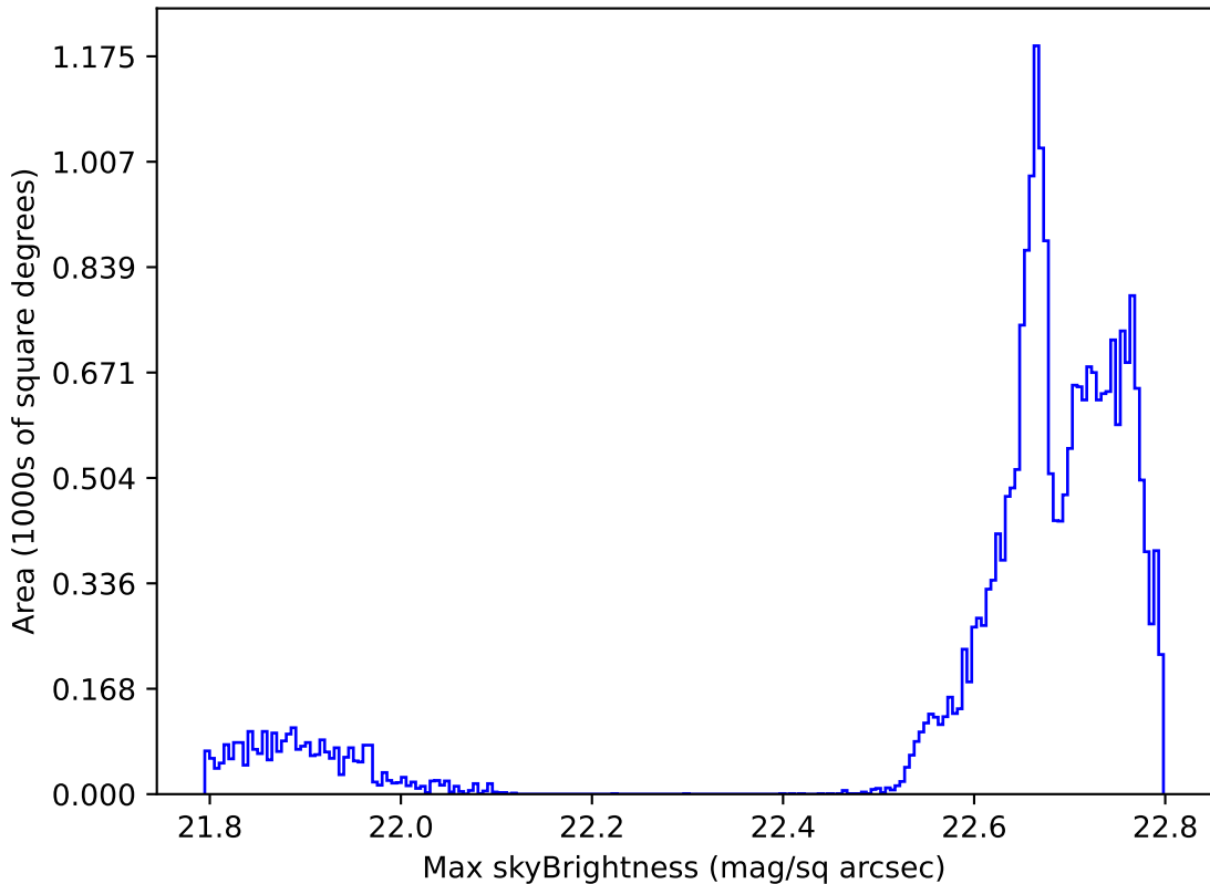
weather_cloudso35v3.4_10yrs All sky all bands: Max skyBrightness
