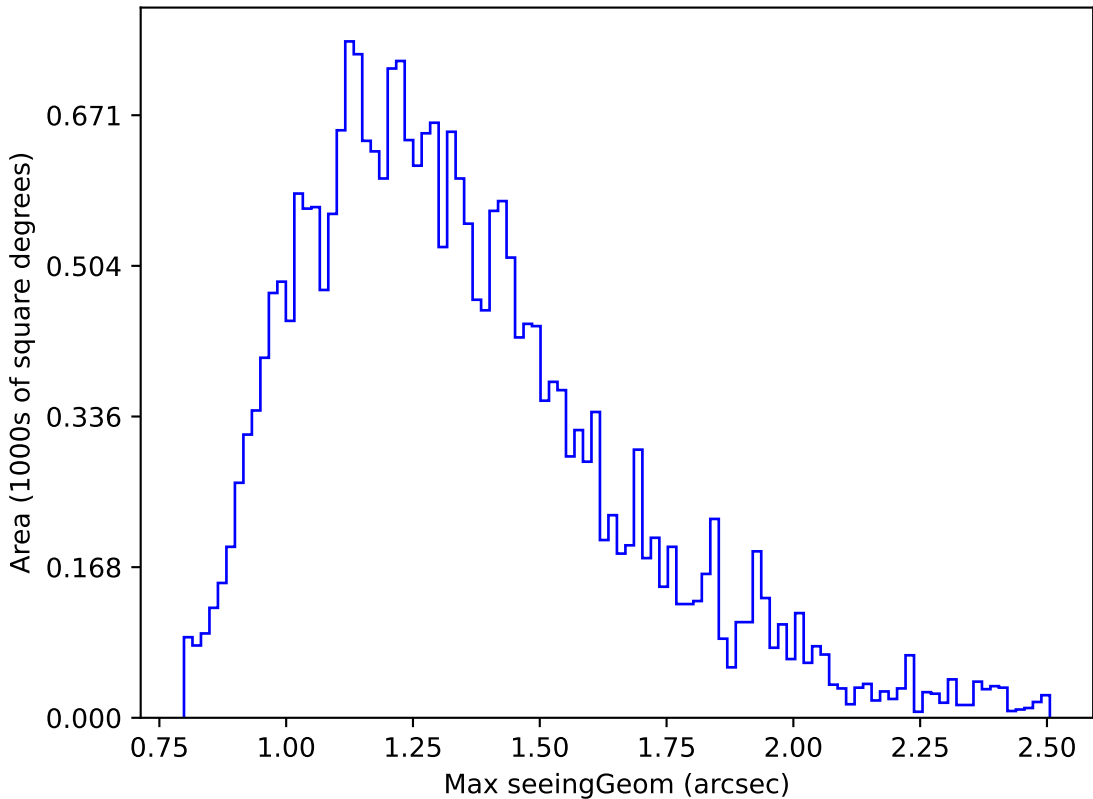
weather_cloudso35v3.4_10yrs Yr 1 z band: Max seeingGeom
