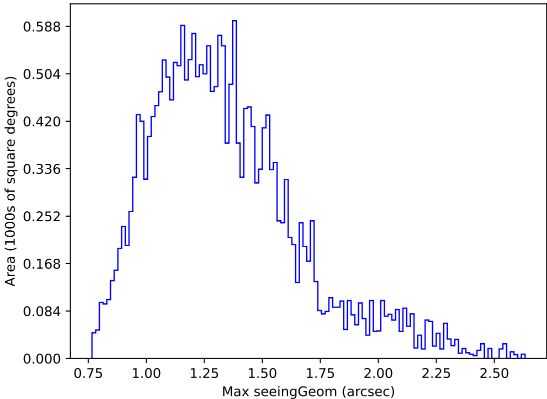
weather_cloudso35v3.4_10yrs Yr 1 u band: Max seeingGeom
