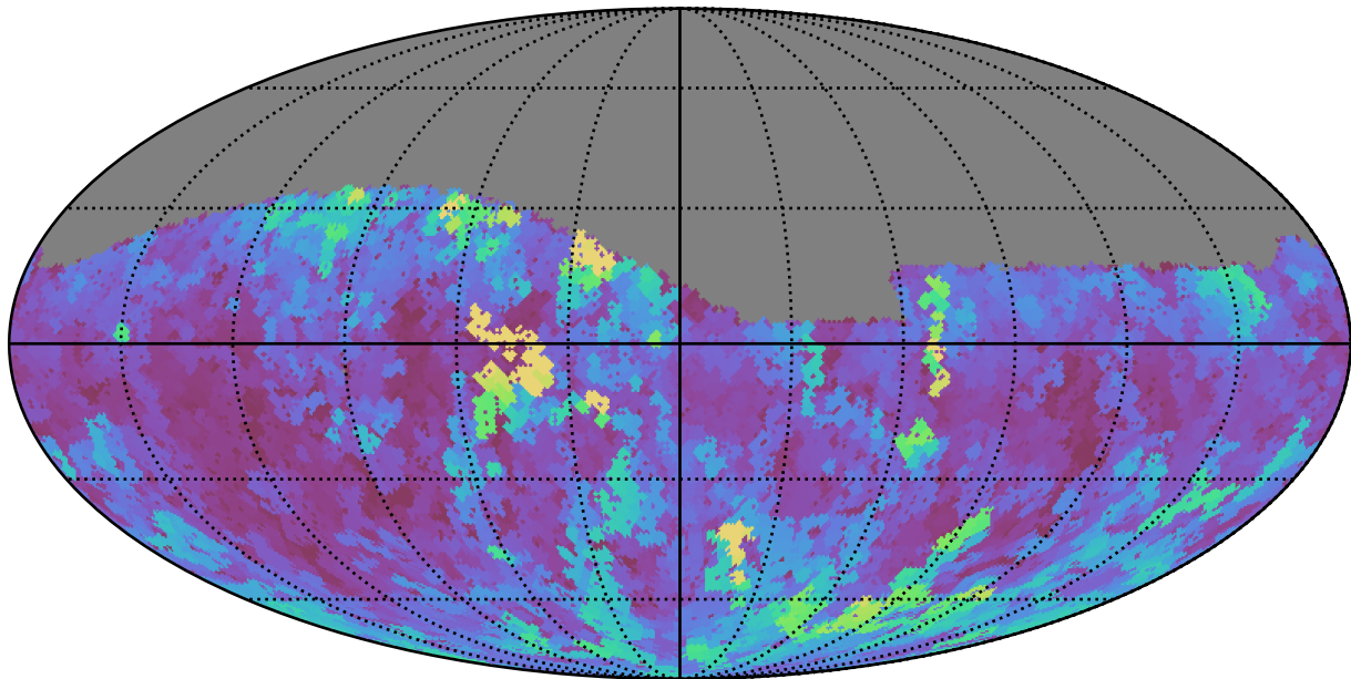
weather_cloudso35v3.4_10yrs Yr 1 g band: Max seeingGeom
