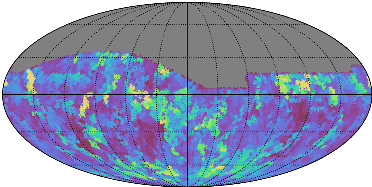
weather_cloudso35v3.4_10yrs Yr 1 all bands: Max seeingGeom
