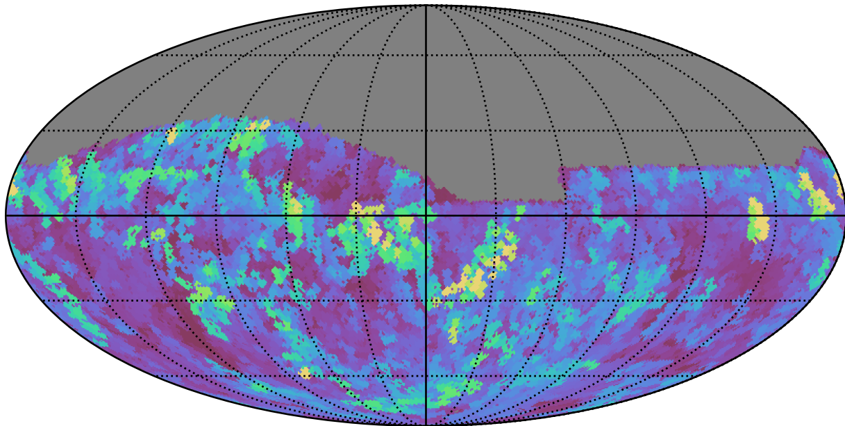
weather_cloudso35v3.4_10yrs Yr 1 z band: Max seeingEff
