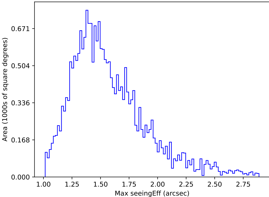
weather_cloudso35v3.4_10yrs Yr 1 y band: Max seeingEff
