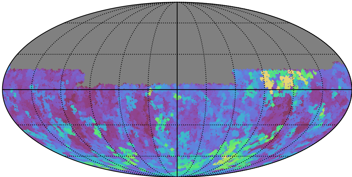
weather_cloudso35v3.4_10yrs Yr 1 u band: Max seeingEff
