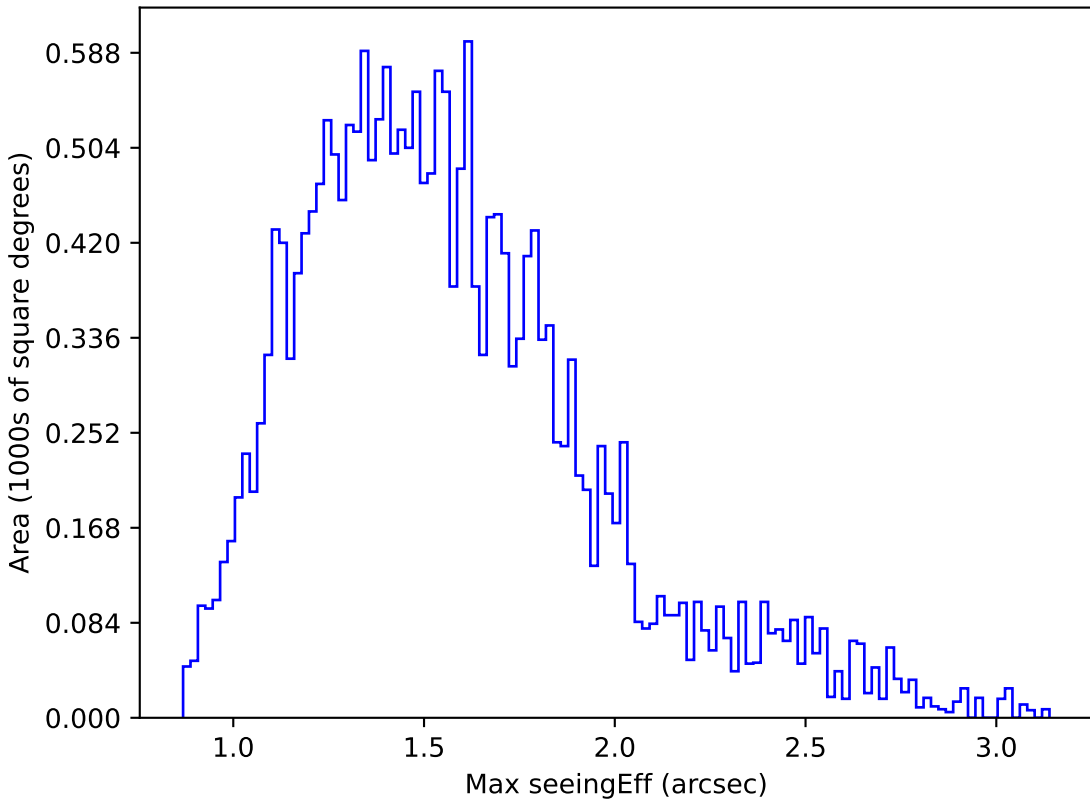
weather_cloudso35v3.4_10yrs Yr 1 u band: Max seeingEff
