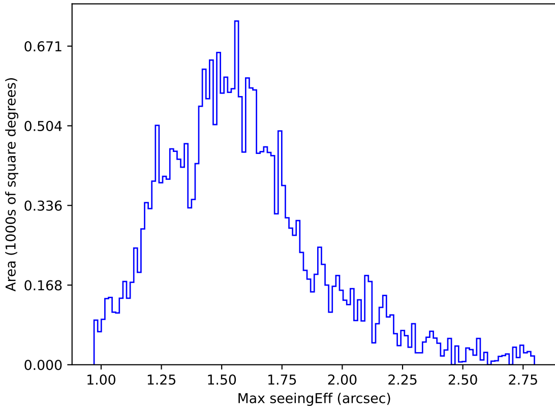
weather_cloudso35v3.4_10yrs Yr 1 r band: Max seeingEff
