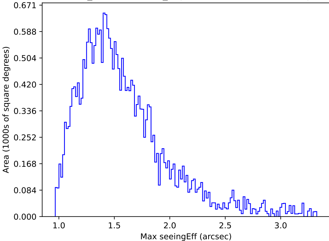
weather_cloudso35v3.4_10yrs Yr 1 i band: Max seeingEff
