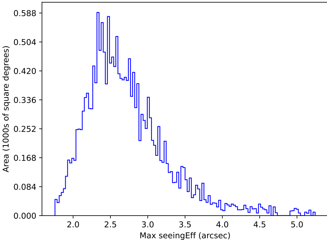
weather_cloudso35v3.4_10yrs WFD z band: Max seeingEff
