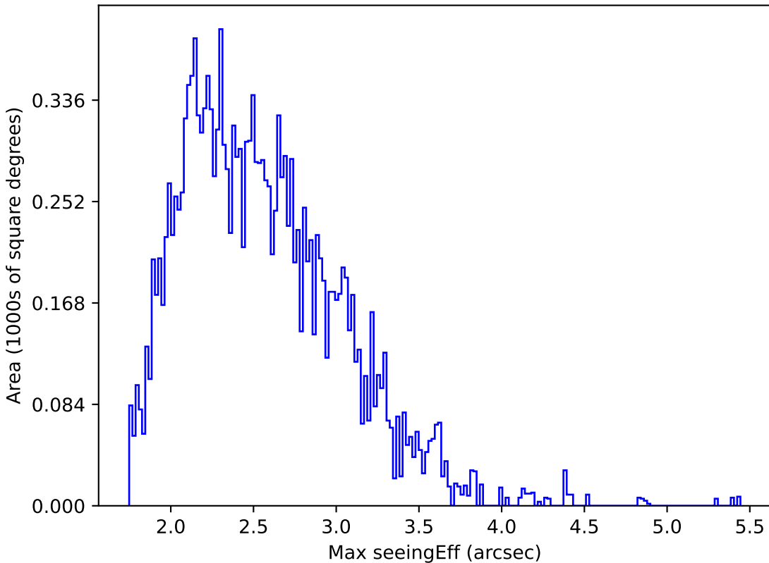
weather_cloudso35v3.4_10yrs WFD y band: Max seeingEff
