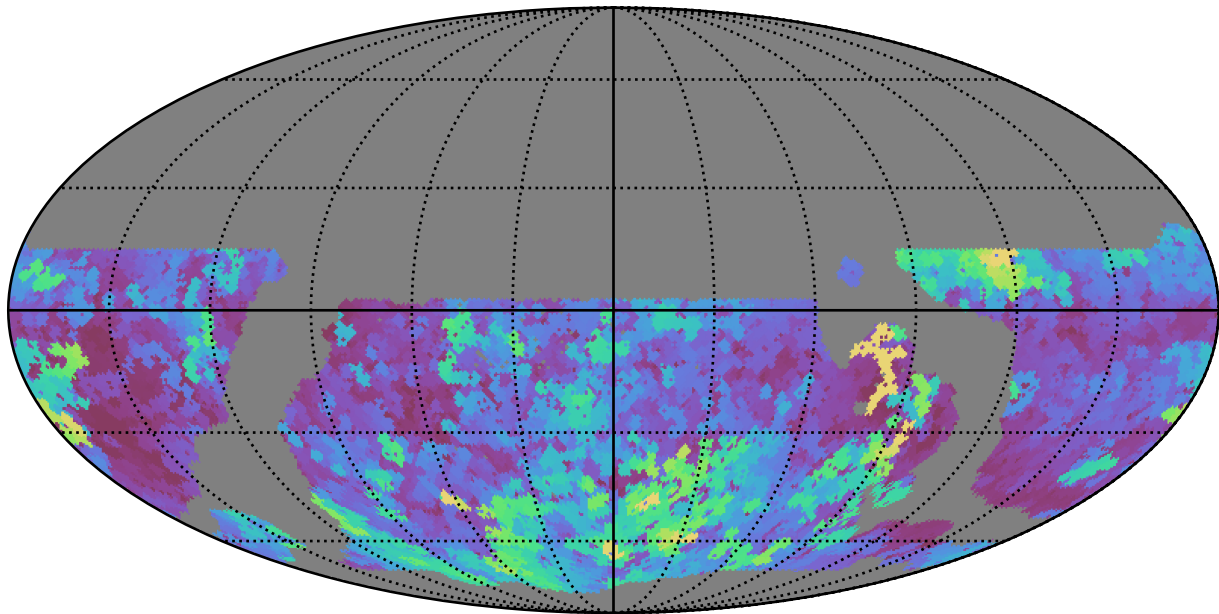
weather_cloudso35v3.4_10yrs WFD u band: Max seeingEff
