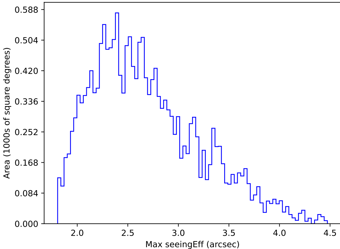
weather_cloudso35v3.4_10yrs WFD u band: Max seeingEff
