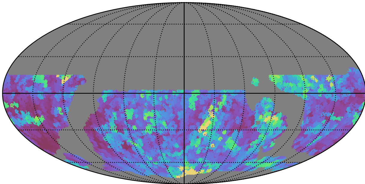
weather_cloudso35v3.4_10yrs WFD r band: Max seeingEff
