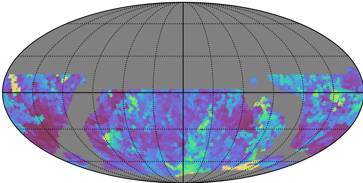
weather_cloudso35v3.4_10yrs WFD all bands: Max seeingEff
