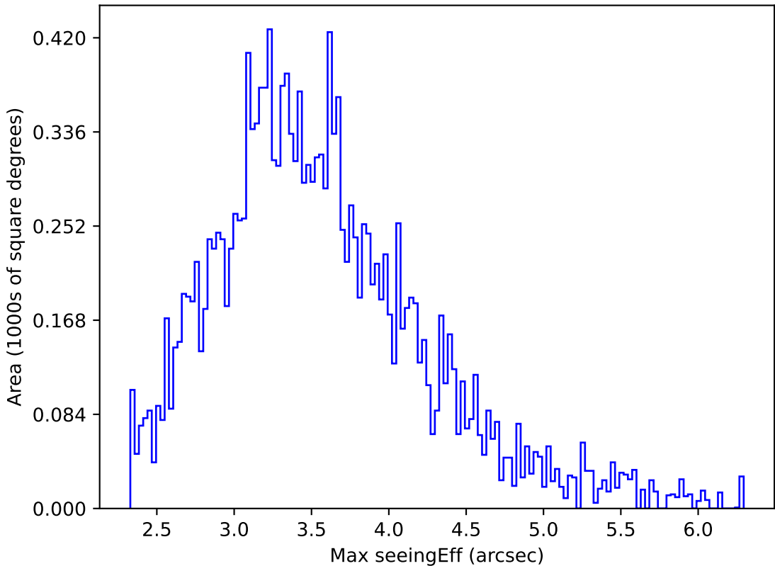
weather_cloudso35v3.4_10yrs WFD all bands: Max seeingEff
