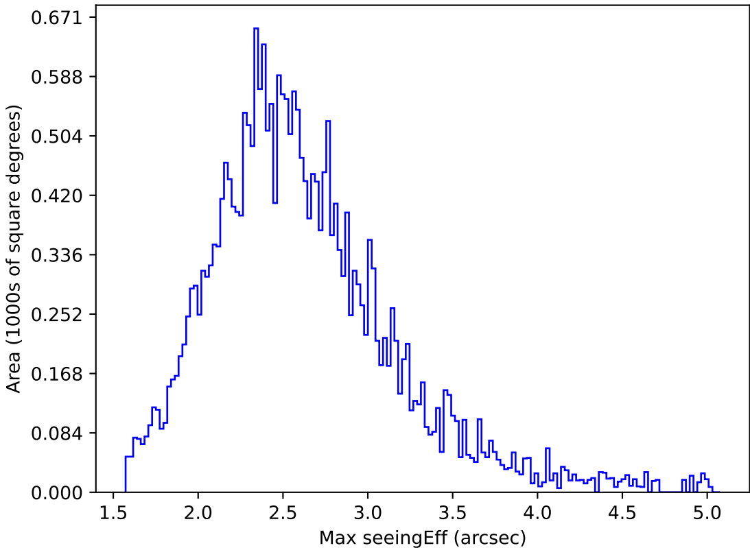
weather_cloudso35v3.4_10yrs All sky z band: Max seeingEff
