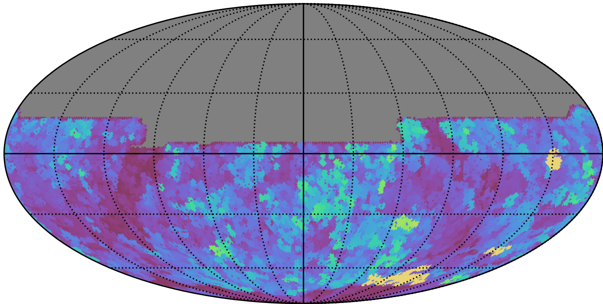
weather_cloudso35v3.4_10yrs All sky y band: Max seeingEff
