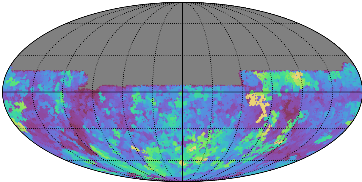
weather_cloudso35v3.4_10yrs All sky u band: Max seeingEff
