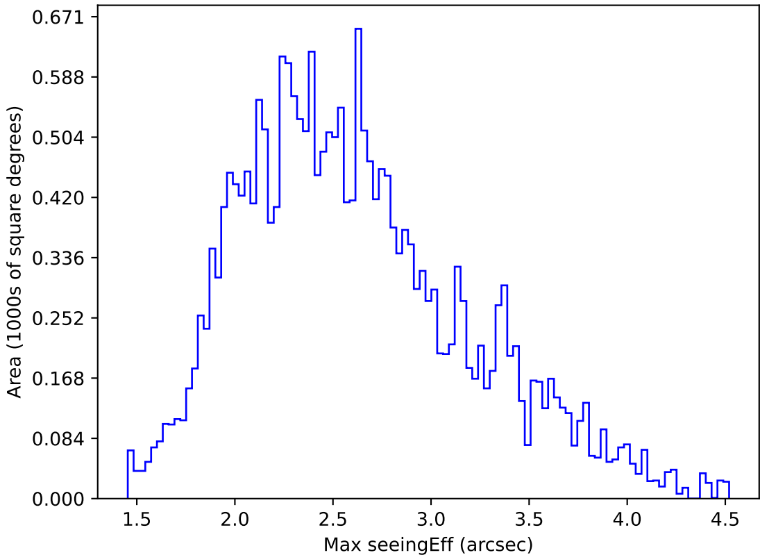
weather_cloudso35v3.4_10yrs All sky u band: Max seeingEff
