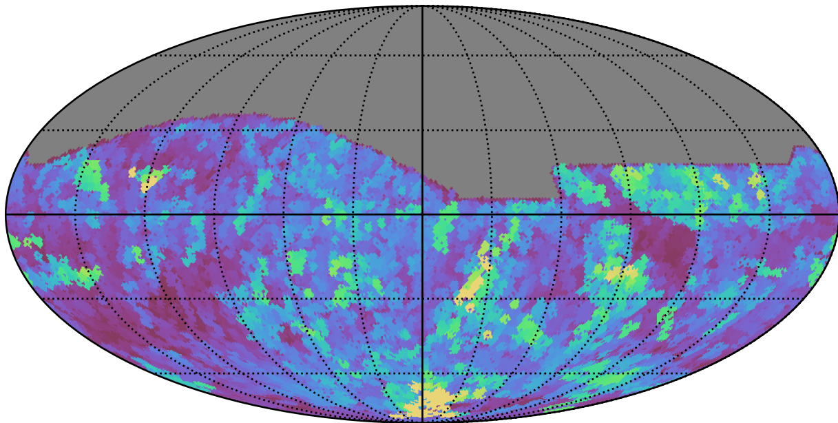
weather_cloudso35v3.4_10yrs All sky r band: Max seeingEff
