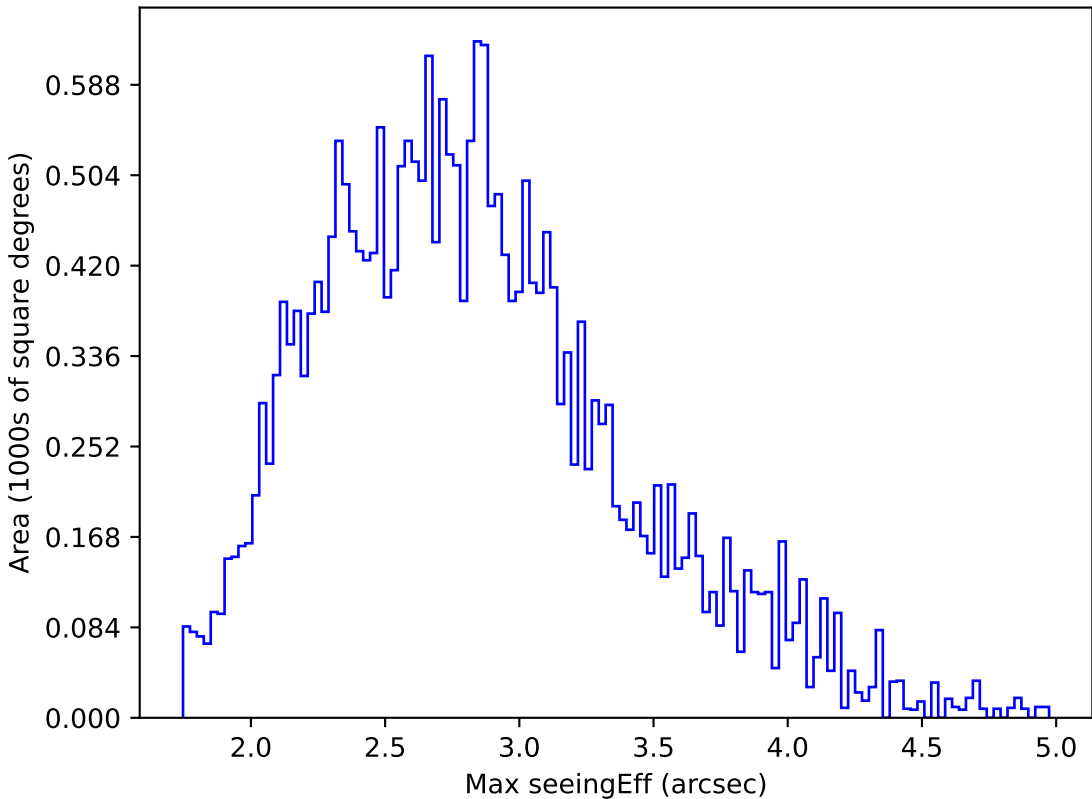
weather_cloudso35v3.4_10yrs All sky r band: Max seeingEff
