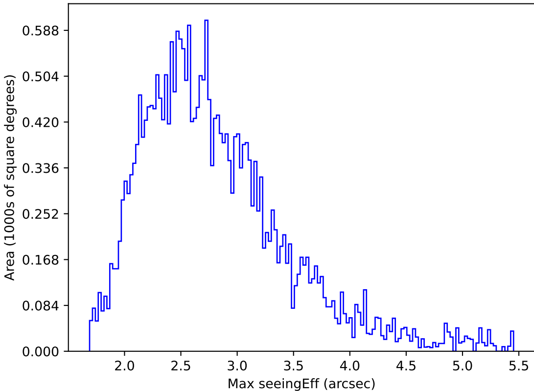
weather_cloudso35v3.4_10yrs All sky i band: Max seeingEff
