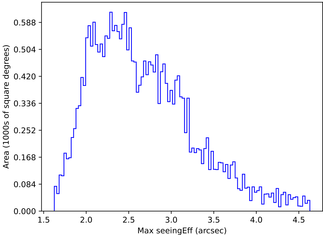
weather_cloudso35v3.4_10yrs All sky g band: Max seeingEff
