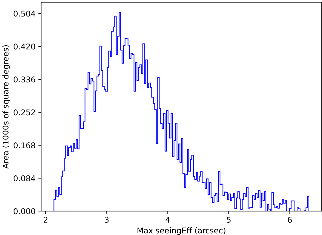
weather_cloudso35v3.4_10yrs All sky all bands: Max seeingEff
