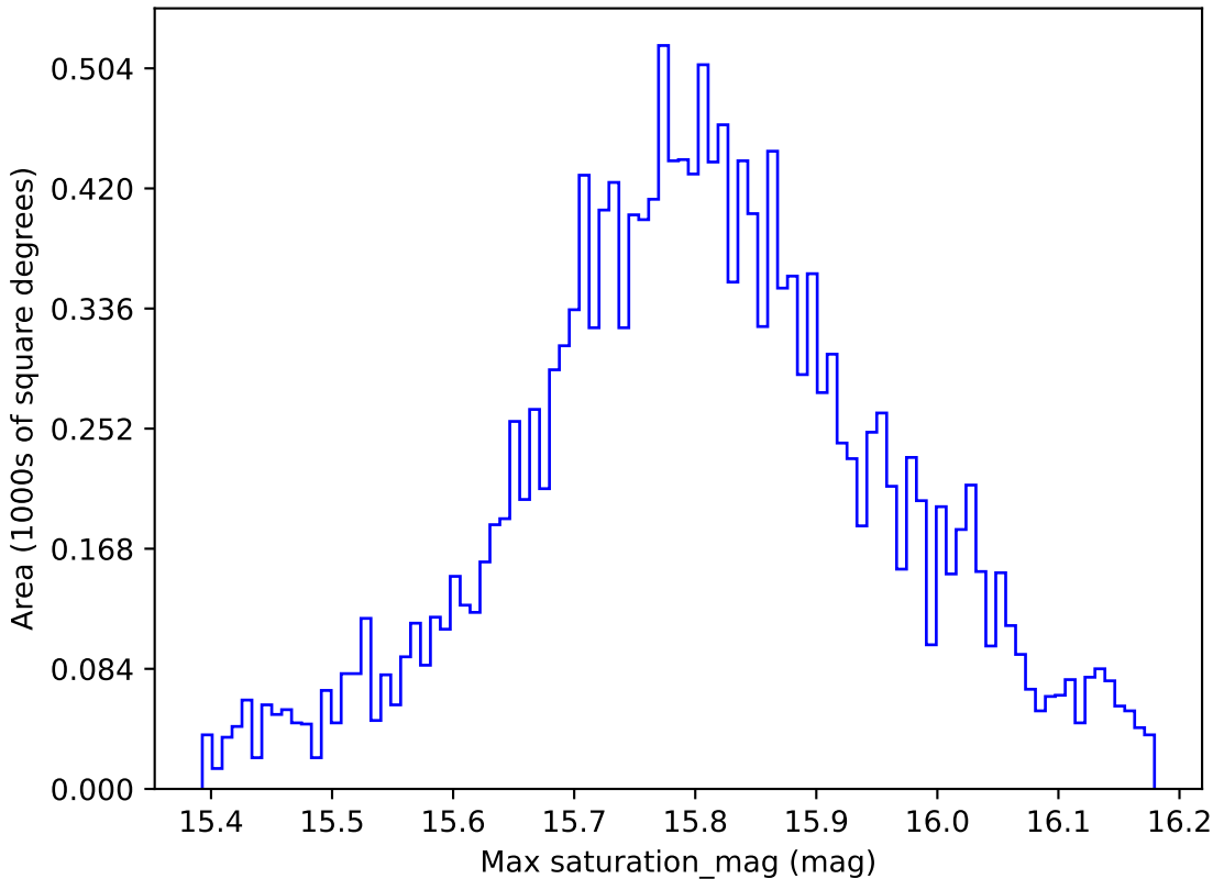
weather_cloudso35v3.4_10yrs WFD all bands: Max saturation_mag
