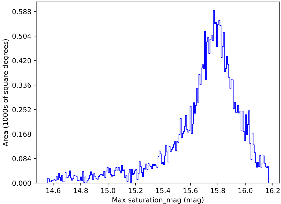
weather_cloudso35v3.4_10yrs All sky all bands: Max saturation_mag
