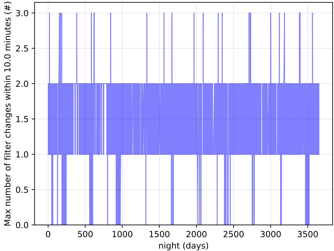
weather_cloudso35v3.4_10yrs Per Night: Max number of filter changes within 10.0 minutes
