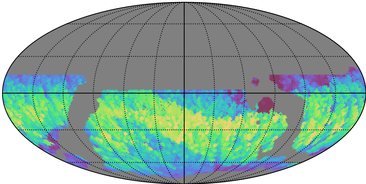
weather_cloudso35v3.4_10yrs WFD z band: Max normairmass
