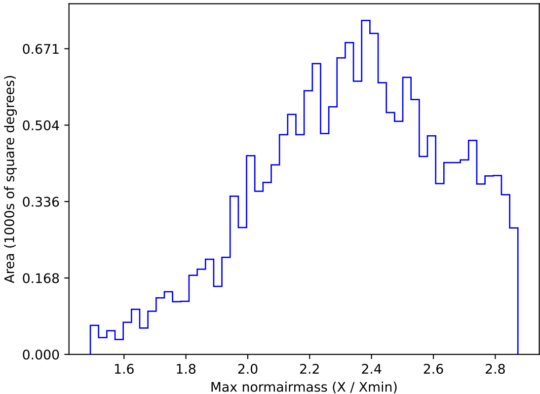
weather_cloudso35v3.4_10yrs WFD z band: Max normairmass
