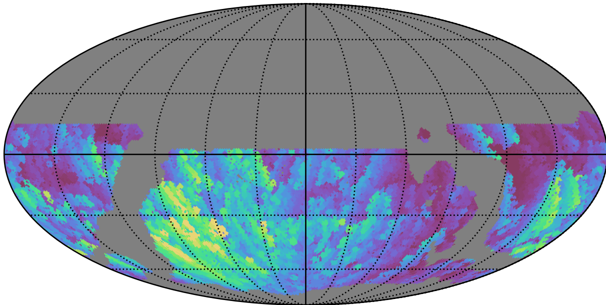
weather_cloudso35v3.4_10yrs WFD u band: Max normairmass
