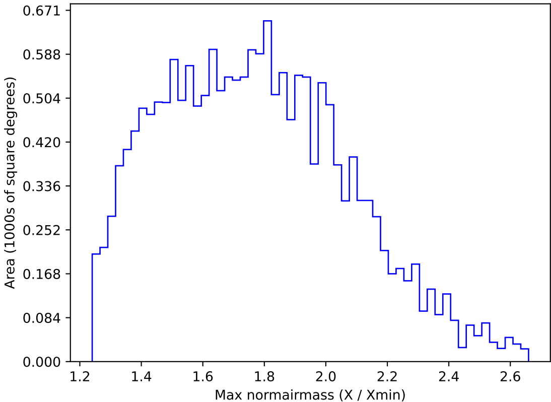
weather_cloudso35v3.4_10yrs WFD u band: Max normairmass
