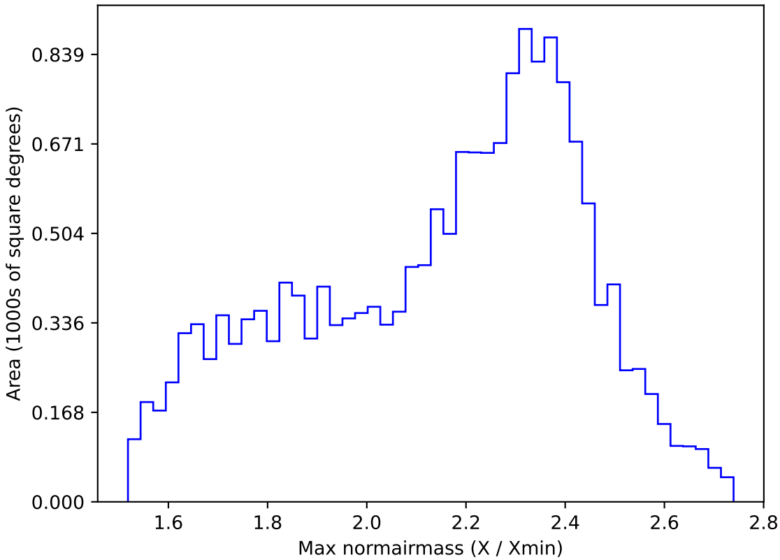
weather_cloudso35v3.4_10yrs WFD r band: Max normairmass
