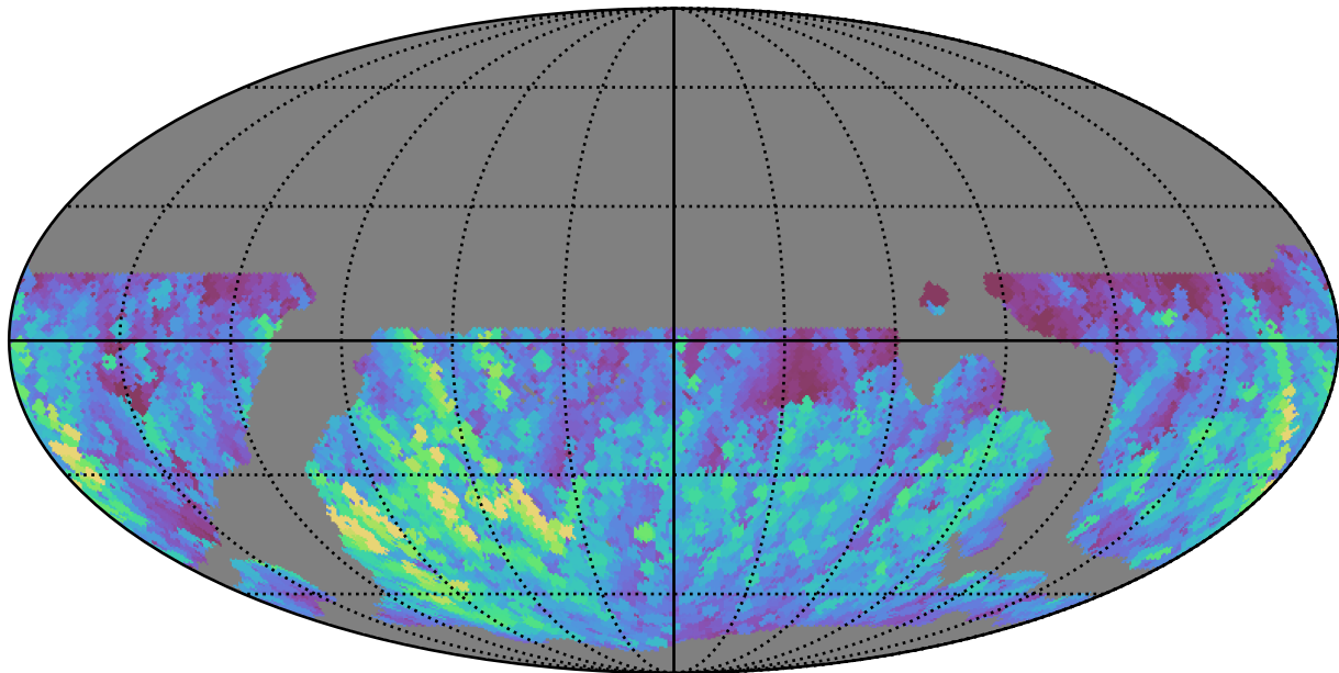
weather_cloudso35v3.4_10yrs WFD g band: Max normairmass
