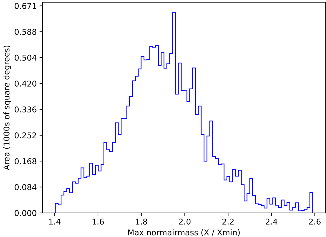
weather_cloudso35v3.4_10yrs WFD g band: Max normairmass
