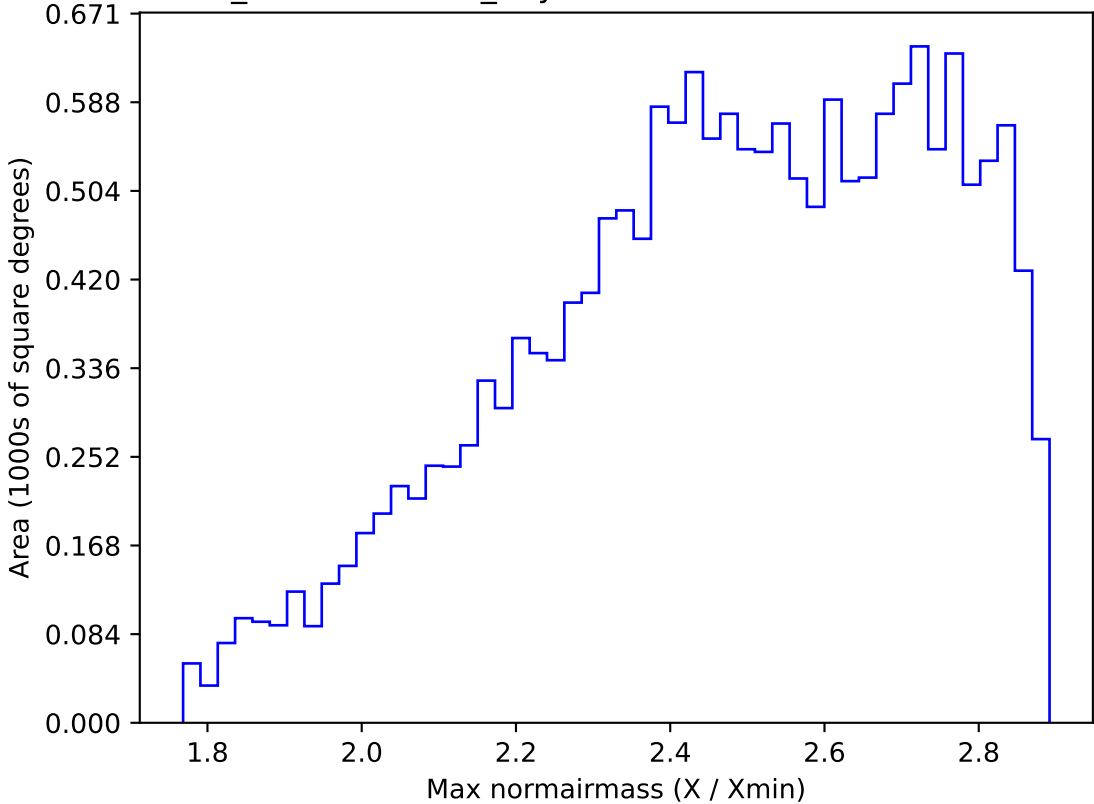
weather_cloudso35v3.4_10yrs WFD all bands: Max normairmass
