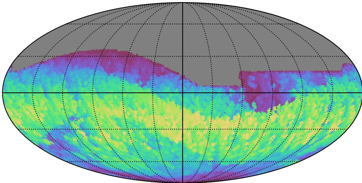
weather_cloudso35v3.4_10yrs All sky z band: Max normairmass
